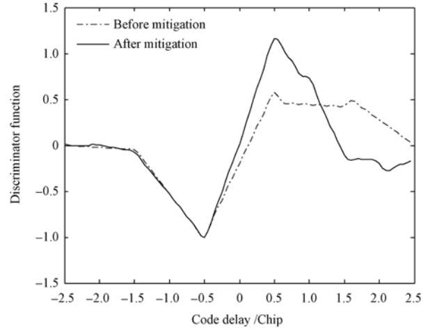
Fig. 7 S-curve in presence of multipath (S-Curve: E-L=1 T_c , BW=10.23\text{MHz} )
